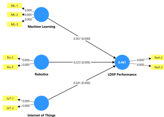
Figure 2: Path Diagram
