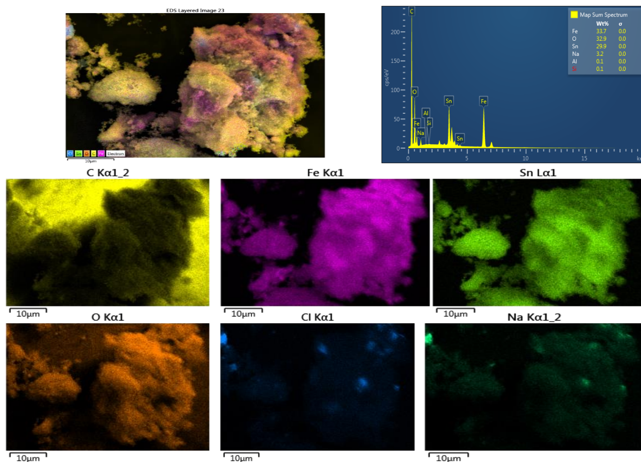
Figure 3: Electron mapping and EDX spectra of \text{SnFe}_2\text{O}_4 .
