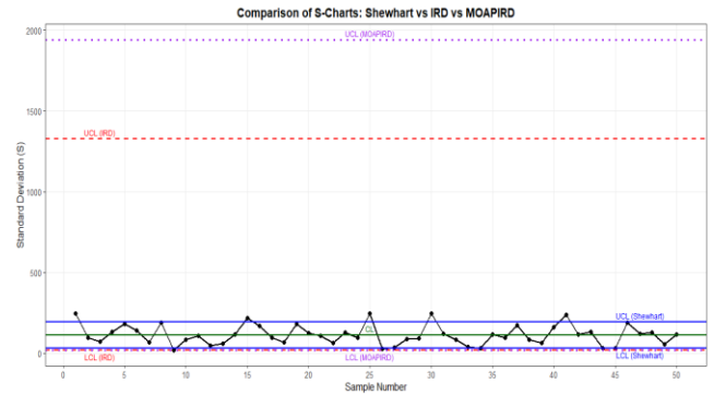
Figure 3: S-Charts for Shewhart, IRD, and MOAPIRD for Thickness of Oil Seal data
